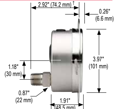
40-400/500 Rear Flange
