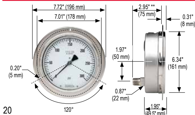
60-410/510 Front Flange
