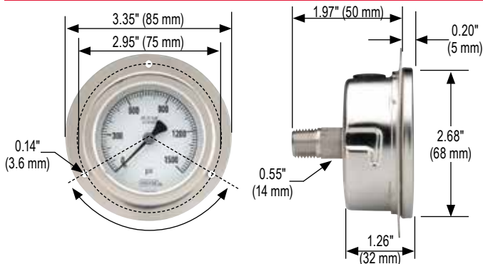
60-410/510 Front Flange
