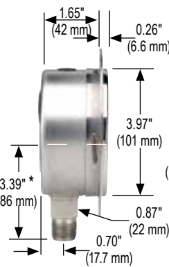
40-400/500 Front Flange
