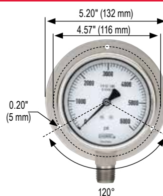
40-400/500 Rear Flange
