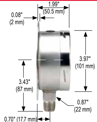
40-400/500 Rear Flange
