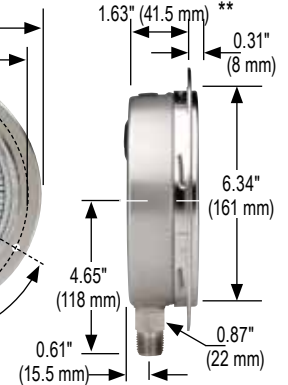
60-400/500 Front Flange
