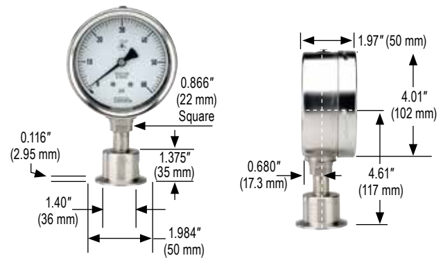
2-1/2" Gauge with 1-1/2" ASME-BPE Sanitary Clamp Connection
