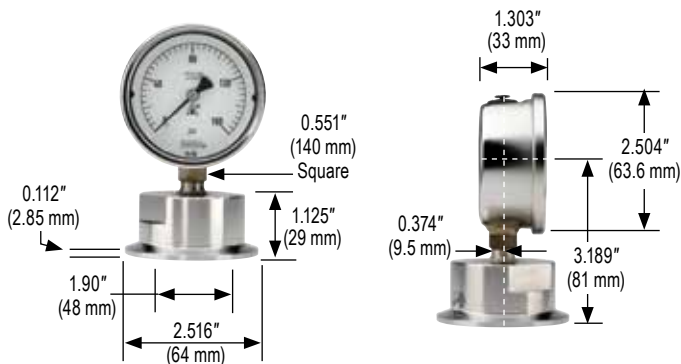
2-1/2" Gauge with 2" ASME-BPE Sanitary Clamp Connection
