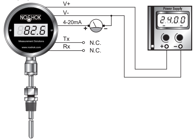
Display and 4-20mA Out
