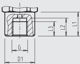
Female thread
